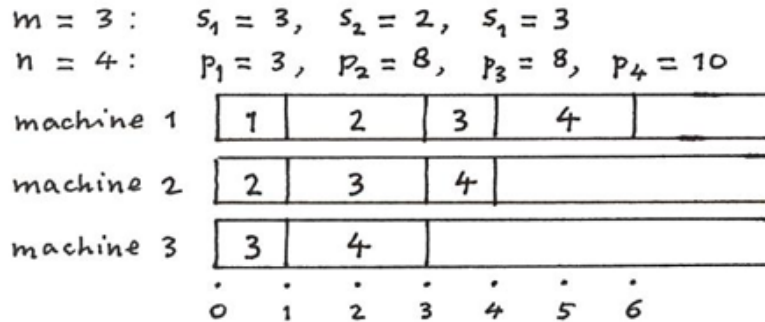
Figure 8.2. Preemptive SPT schedule for Q|pmtn|\sum C_j .
