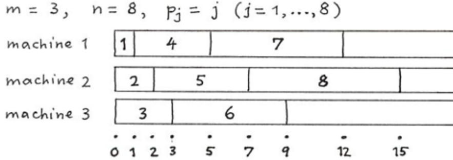
Figure 8.1. An optimal schedule for P||\sum C_j .
